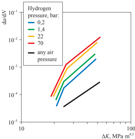
Fig. 4. Impact of different hydrogen pressures on the crack propagation in pipe steel [11]
