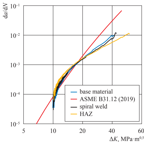
Fig. 10. Result of fracture-mechanical testing on pipeline grade L 485 (medium: 100 bar & 100% hydrogen)
